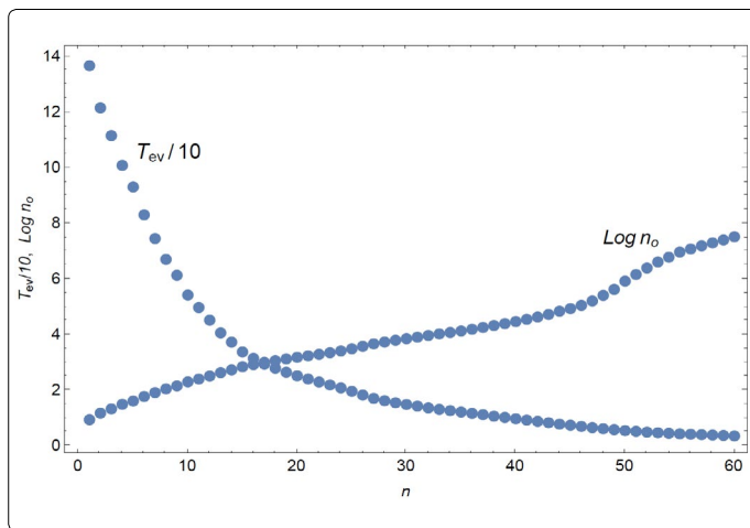
Figure 2. The combined plot of the temperature in eV and the hydrogen plasma density n_o over the region examined for locating the phase-transition.
