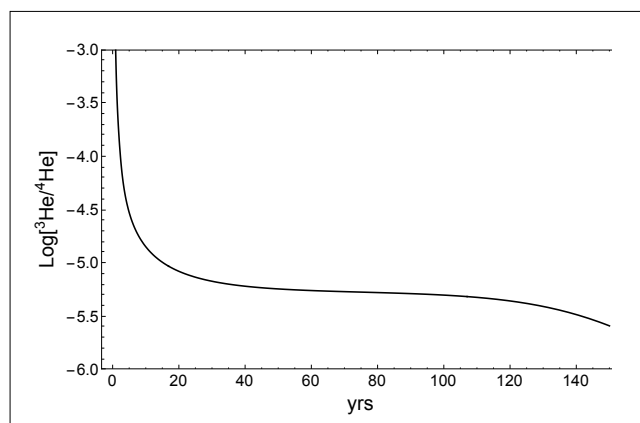
Figure 2. The ratio of ^3\text{He} and ^4\text{He} as a function of time from the numerical integration of the reaction rate equations.
